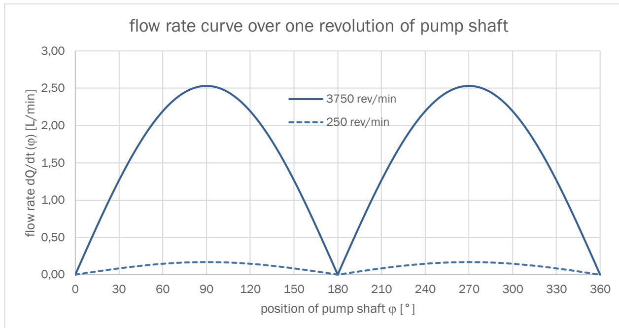
Figure 3 flow rate curve at the high-pressure outlet of the HPP 200
