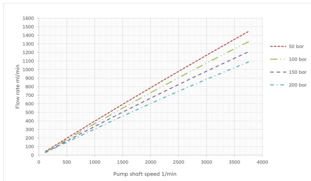
Figure 1 flow rate (water) in dependency of speed pump shaft and pressure with pre-pressure of 2 bar
