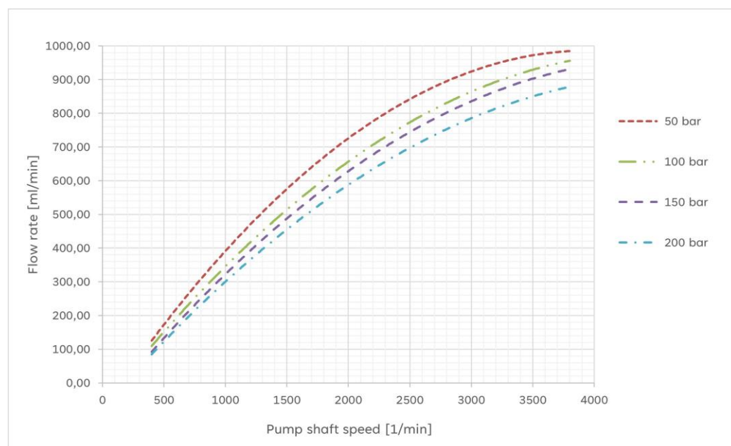
figure 2 flow rate (water) in dependency of speed pump shaft and pressure with pre-pressure of 0 bar
